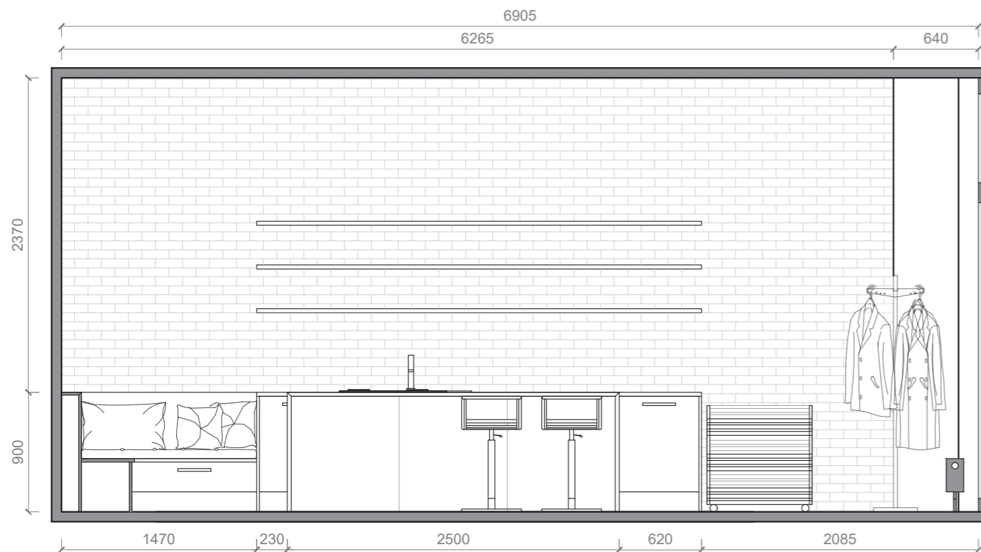
ELEVATION E - KITCHEN FRONT VIEW WITH ISLAND
