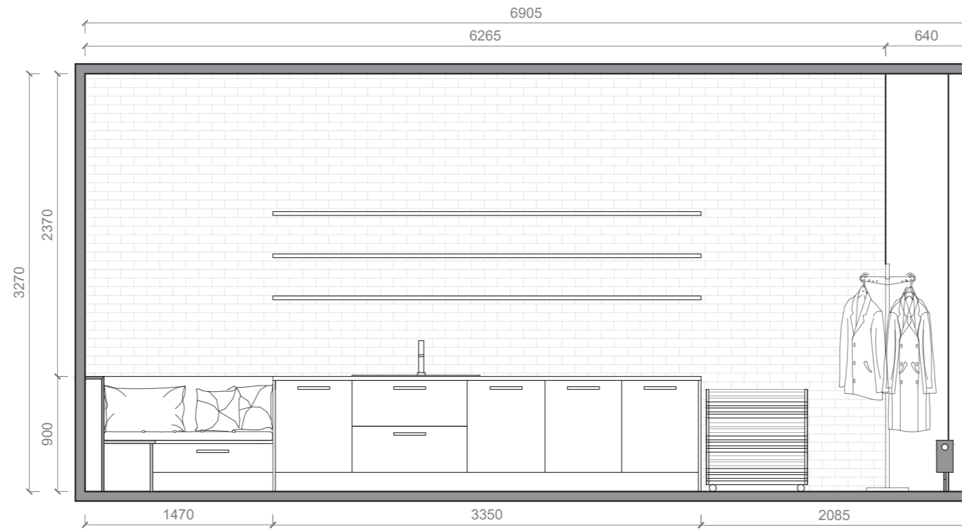
ELEVATION C - KITCHEN ISLAND FRONT SIDE
