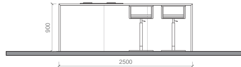
ELEVATION D - KITCHEN ISLAND BACK SIDE
